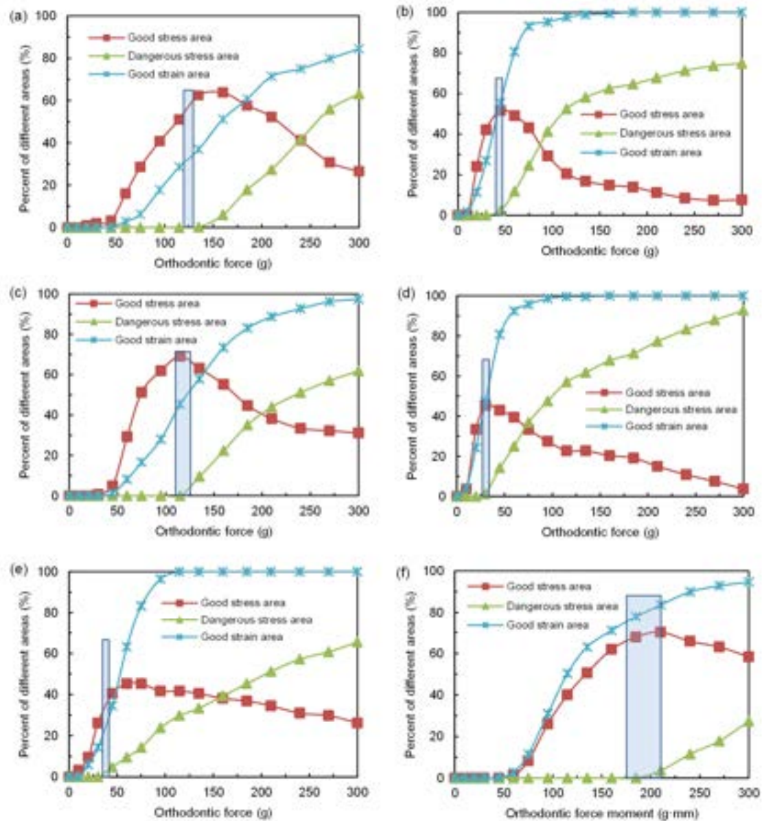
Fig. 3 Percentages of good stress areas, dangerous stress areas, and good strain areas with the change of the orthodontic force or force moment
