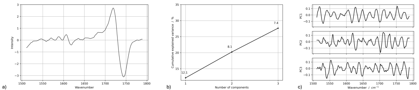
Fig 15. Raman PCA summary for Tera Harz TC-85 DAC aligners. (a) Average first-derivative Raman spectrum in the 1500–1800 cm -1 region. (b) Cumulative explained variance for the first three principal components. (c) Loadings of PC1-PC3 highlighting the main contributions of aromatic C=C and ester/urethane C=O bands.
