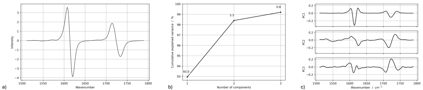
Fig 16. Raman PCA summary for SmartTrack™ Invisalign® aligners. (a) Average first-derivative Raman spectrum in the 1500–1800 cm -1 region. (b) Cumulative explained variance for the first three principal components. (c) Loadings of PC1-PC3 showing contributions from the same polyurethane-related bands and the absence of new features after intraoral exposure.
