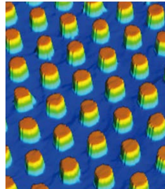
Wafer Bumps
